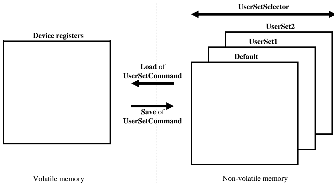
Figure 21 – UserSetSelector / UserSetCommand
