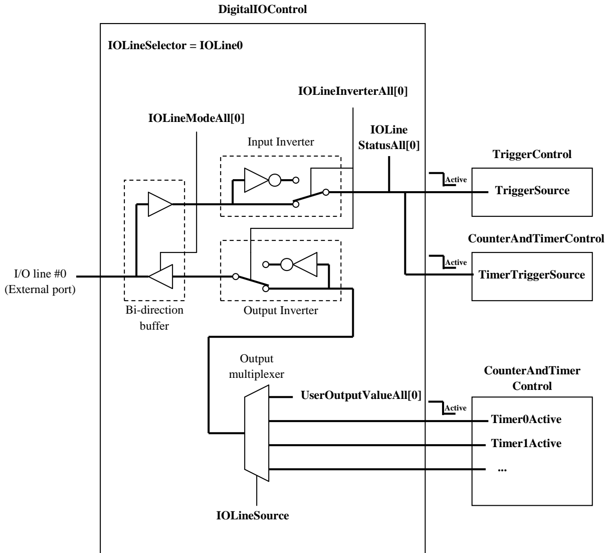
Figure 22 – Block diagram of DigitalIOControl
