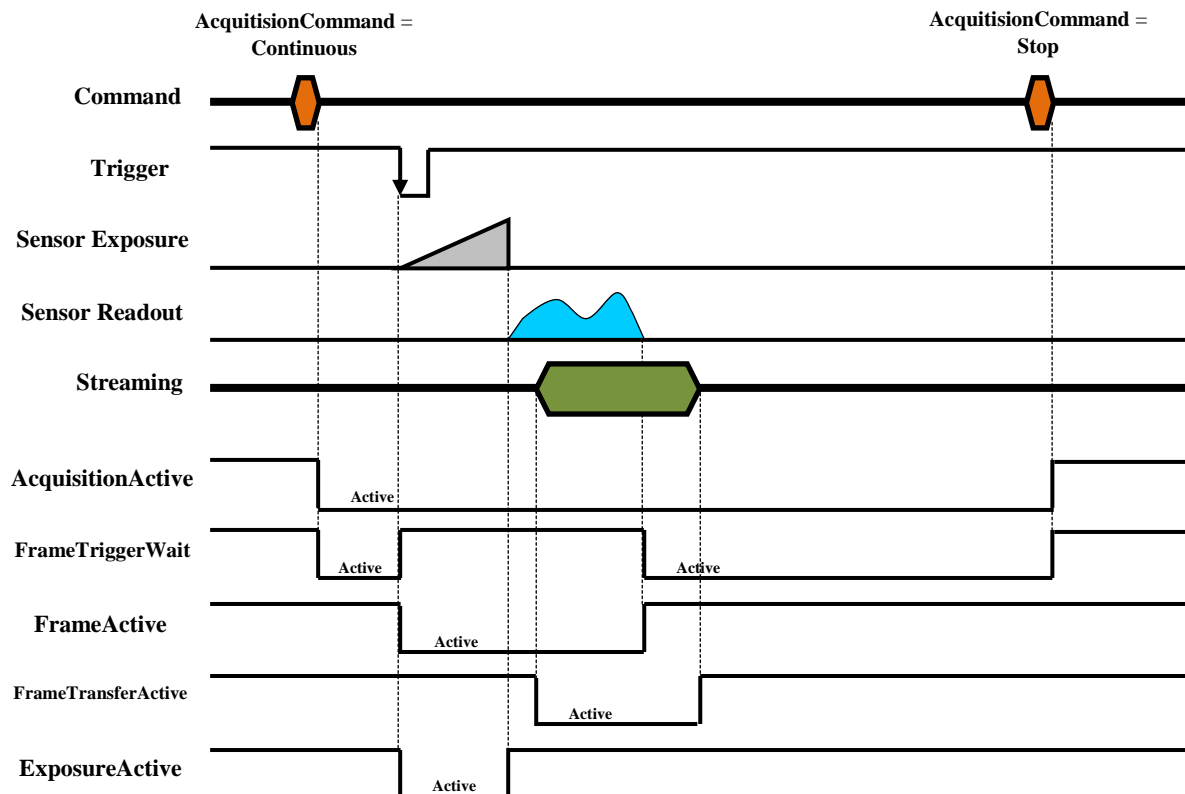
Figure 23 – Output signal definition
