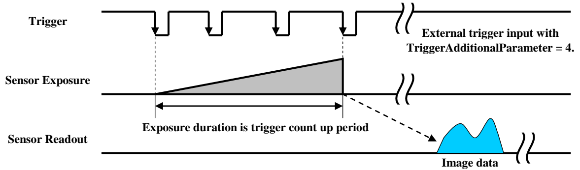
Figure 15 – Trigger Sequence2
