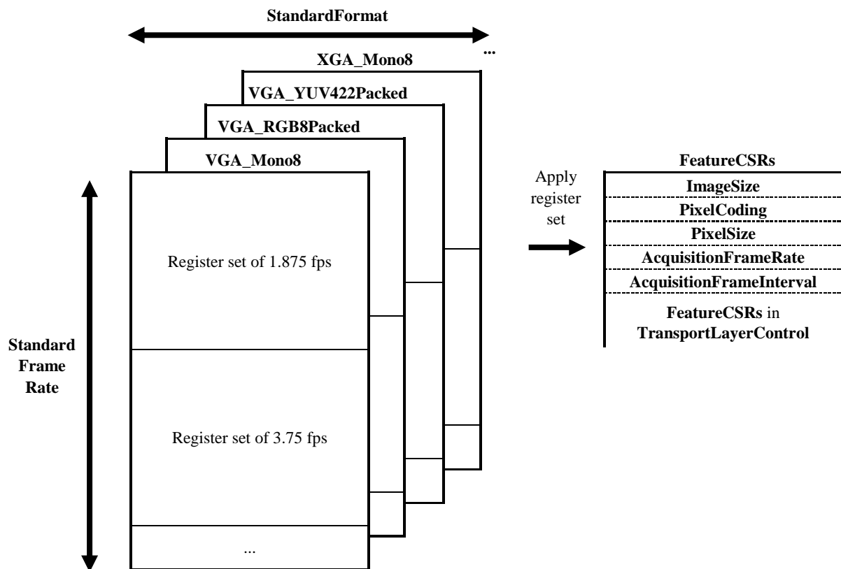
Figure 20 – StandardFormat / StandardFrameRate
