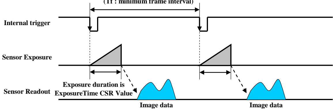
Figure 16 – Trigger Sequence3
