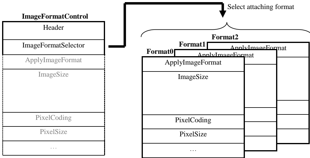
Figure 9 – ImageFormatSelector
